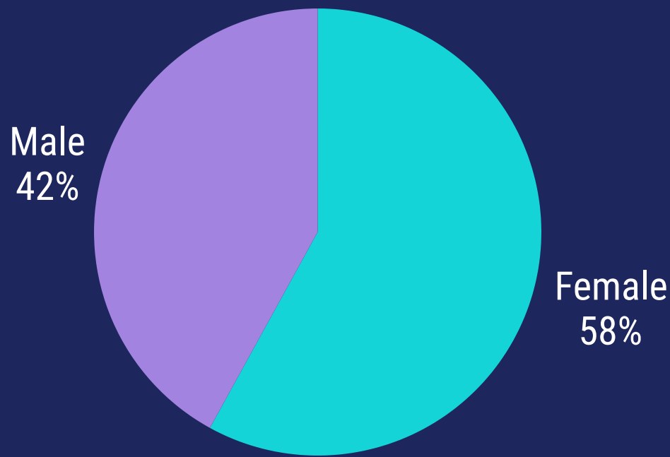
Gender
