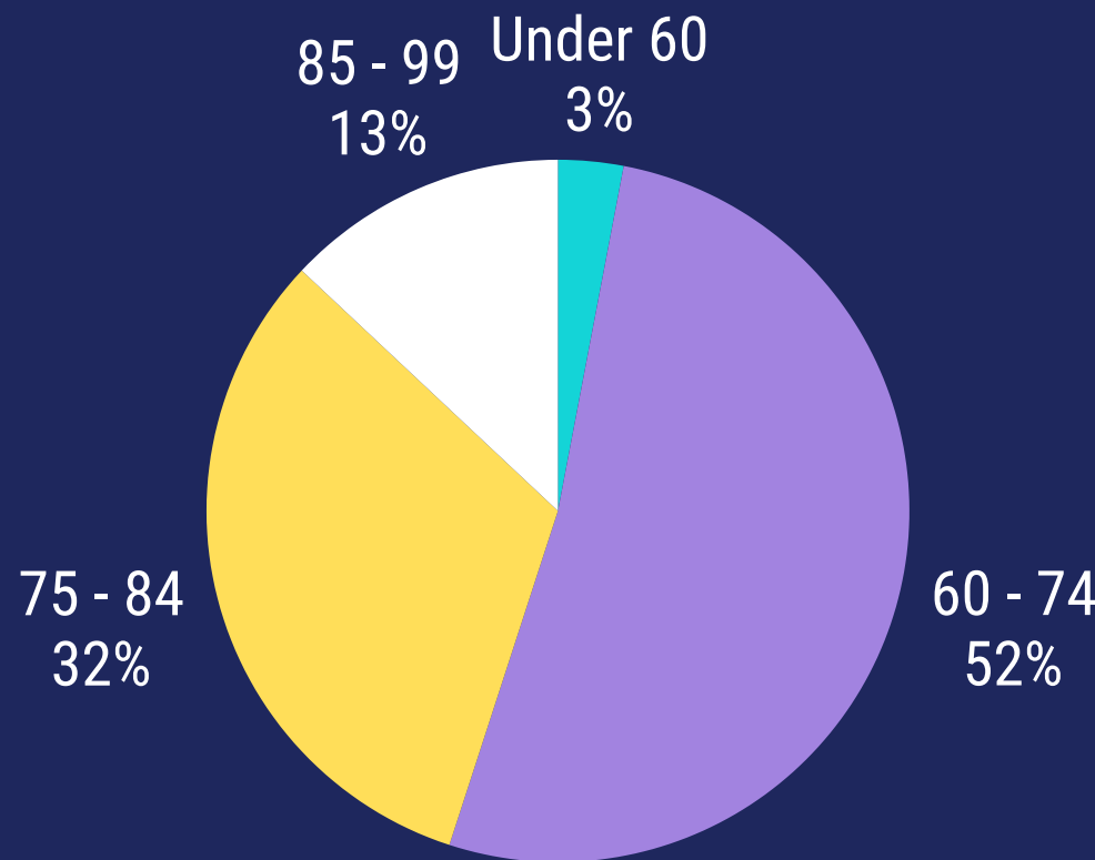
Age
