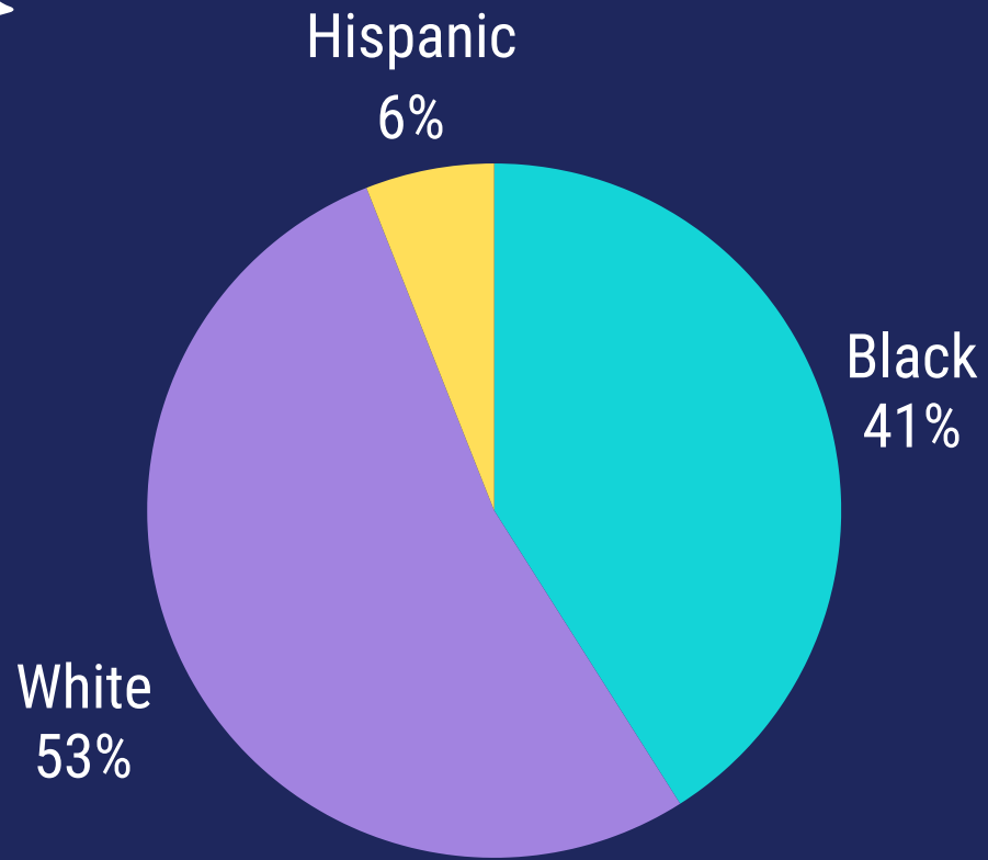
Race / Ethnicity
